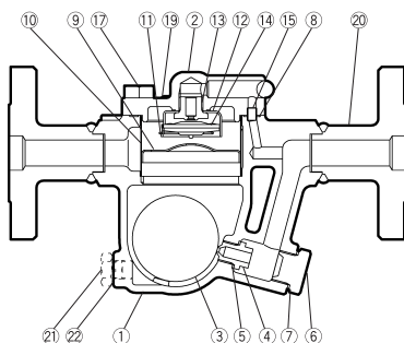
JH5SL-X
