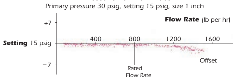
Pressure vs. Flow Rate
