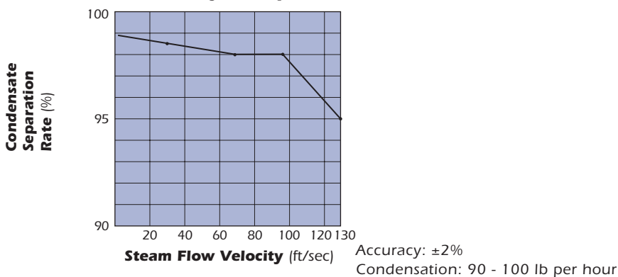
Steam Flow Velocity vs. Separation Rate
