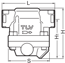
承插焊
